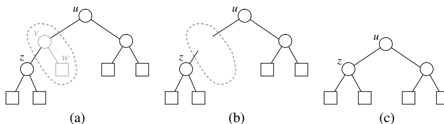
Figure 8.10: Operation that removes an external node and its parent node, used in the justification of Proposition 8.9.
